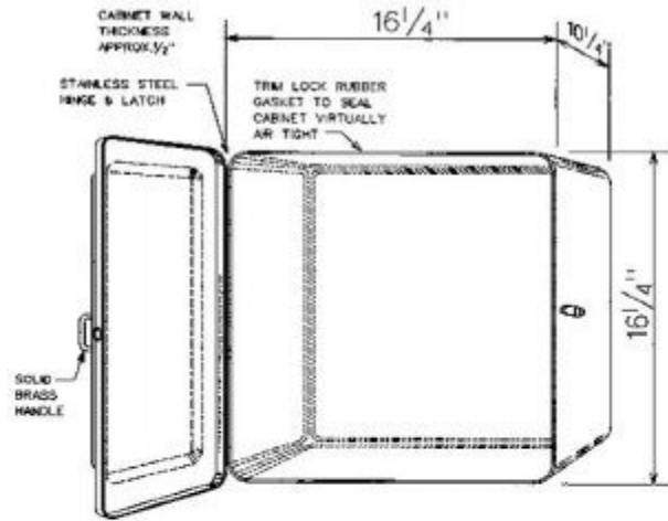
Emergency Fire Blanket Cabinet FBC-15
