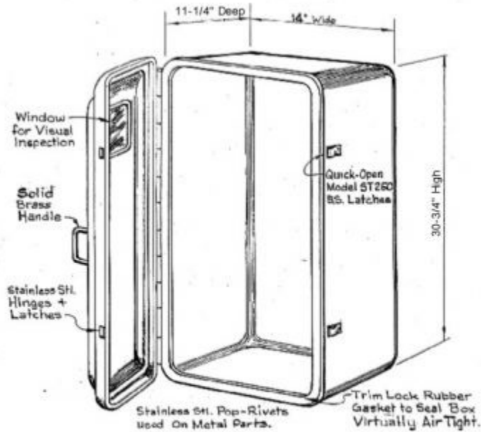
FIRE EXTINGUISHER CABINET for 20 lb or 30 lb Cartridge Operated or Stored Pressure Extinguishers up to 30 in Tall. F. E. B. 30
