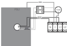
Typical wiring diagram - WL168-HO
