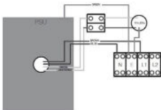
Typical wiring diagram - WL168-HO
